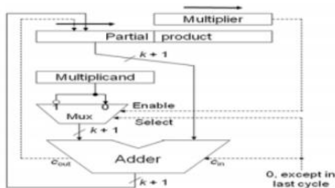
Fig6: Baugh-wooley multiplier block diagram
