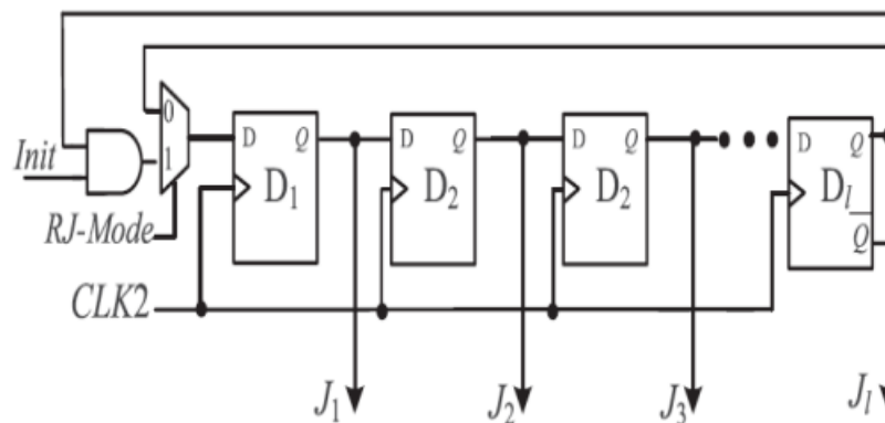
Figure4: Reconfigurable Johnson counter.
