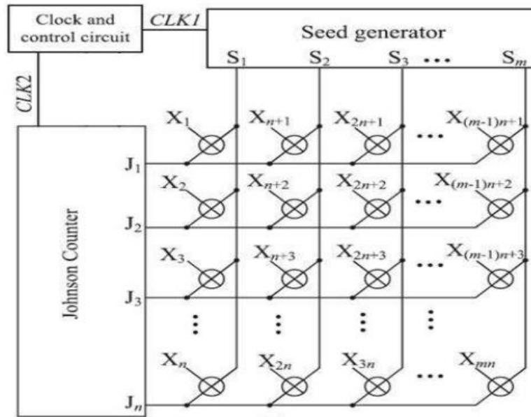
Figure5: MSIC-TPGs for test-per-clock scheme
