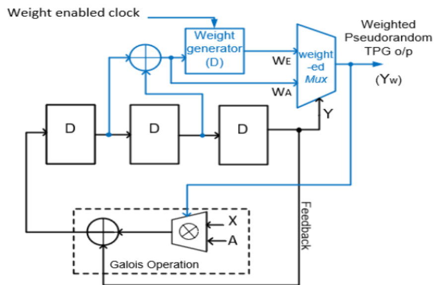
FIGURE1. Proposed 3-bit weighted pseudorandom TPG
